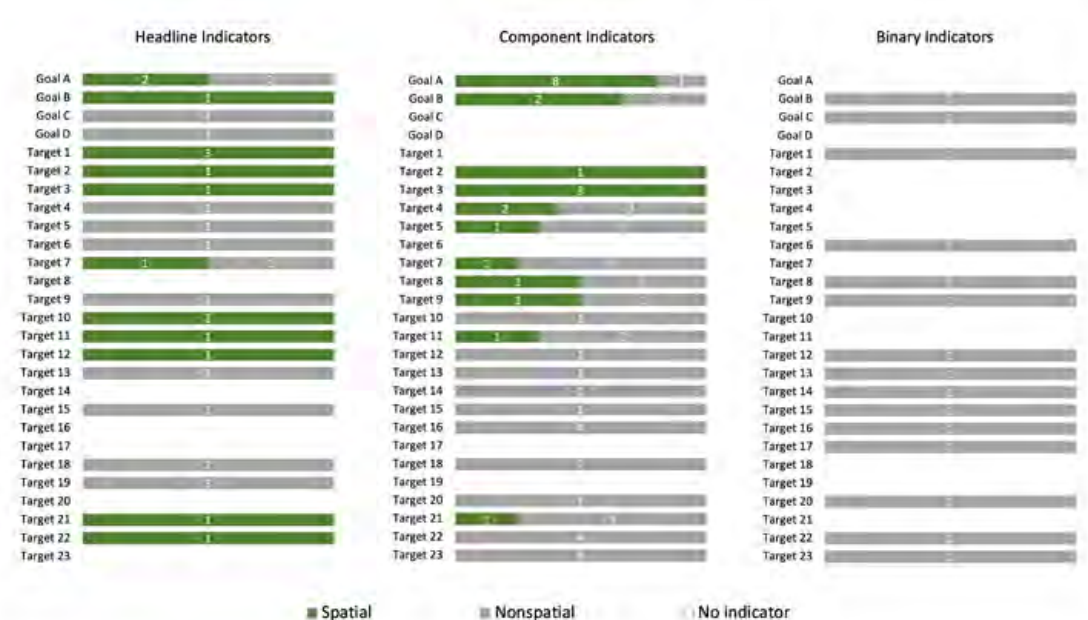
Figure 1. Identification of the number of Kunming-Montreal Global Biodiversity Framework headline and component indicators per goal/target that encourage the use of spatial data for the calculation of the indicator or to provide disaggregated information required by the indicator. Dark green bars indicate spatial indicators, and dark grey non-spatial indicators (see Table 1 for definitions and Annex 1 for a detailed list of indicators). The number within each bar is the number of indicators identified within that class for each goal/target. Goals/Targets with no bar are those for which no indicators have been identified.
